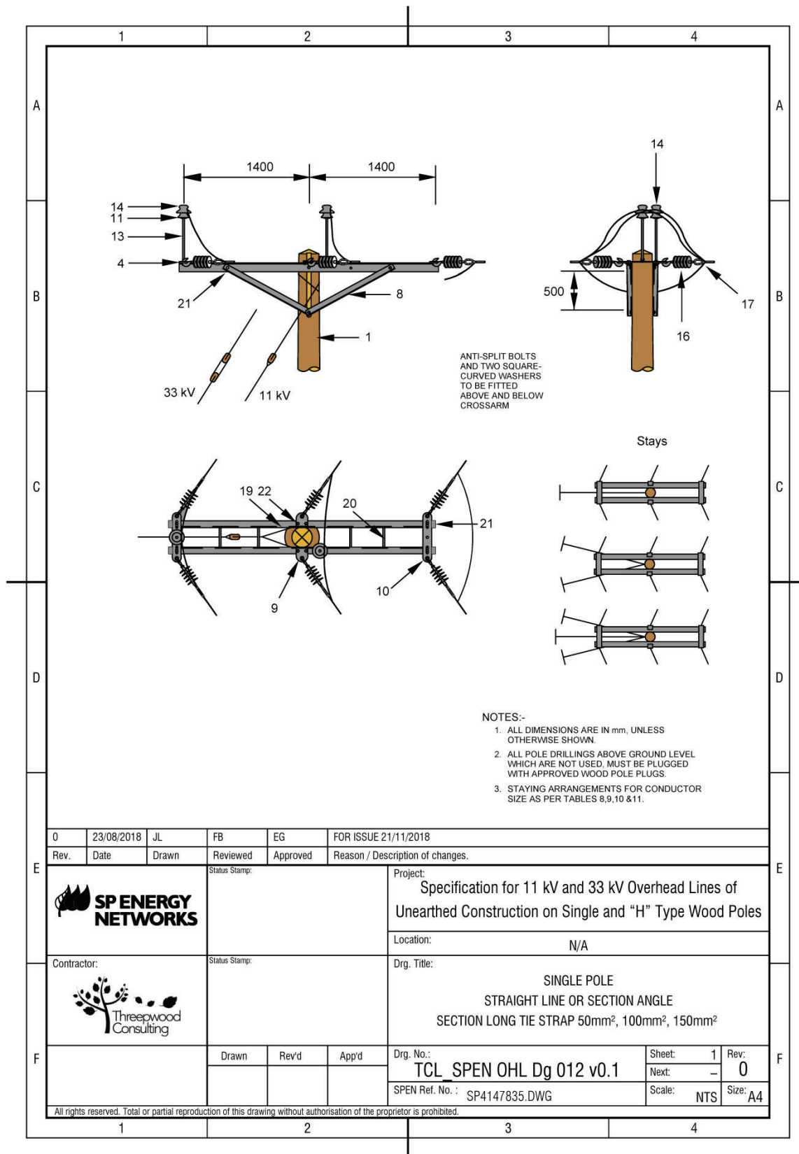
22.12 Figure 12 General Arrangement Single Pole Straight Line or Angle Section Long Tie Strap 50mm 2 , 100mm 2 , 150mm 2 (Drawing No. SP4147835)
